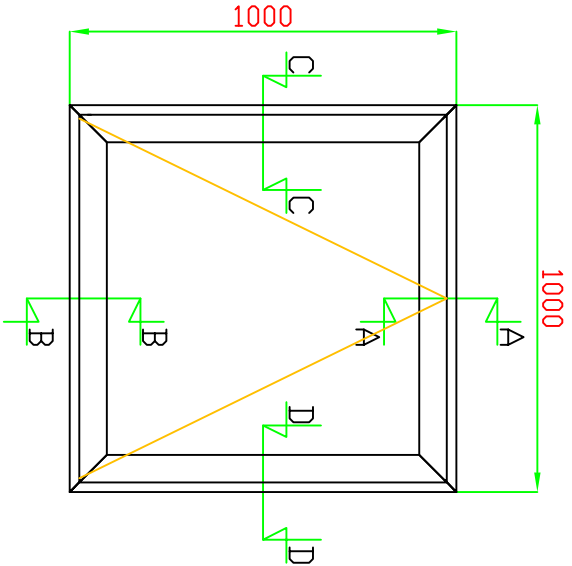
External Elevation
