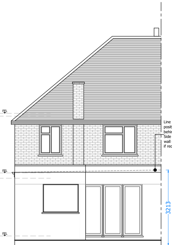
REAR ELEVATION
