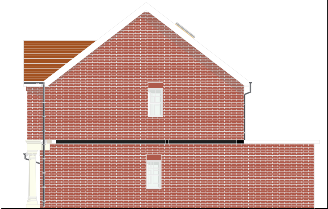
1:100 Proposed Side Extension
