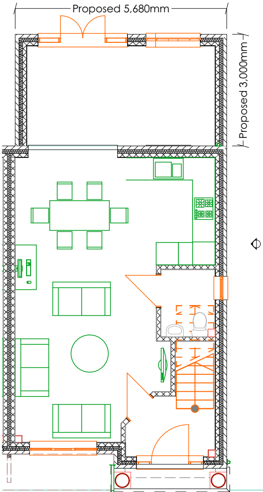
1:100 Proposed Ground Floor Plan
