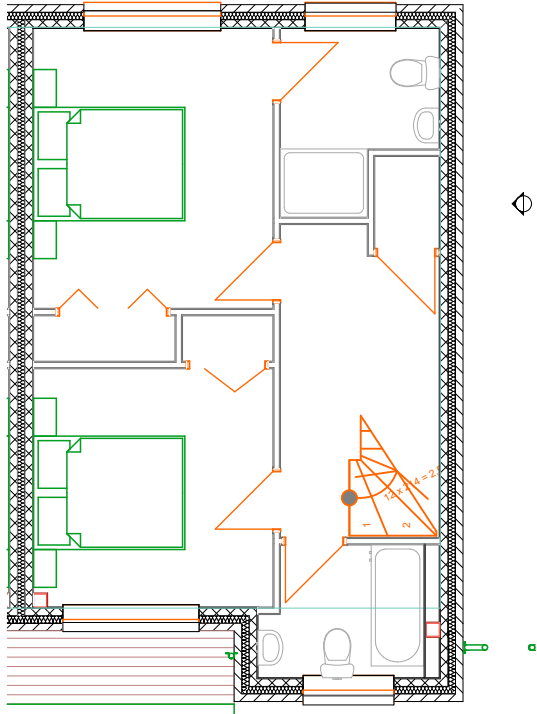
1:100 Existing First Floor Plan
