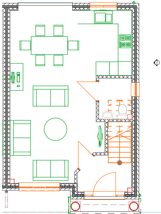
1:100 Existing Ground Floor Plan
