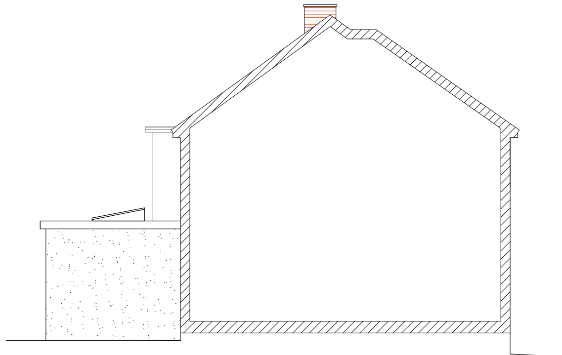
PARTY WALL NORTH WEST ELEVATION
