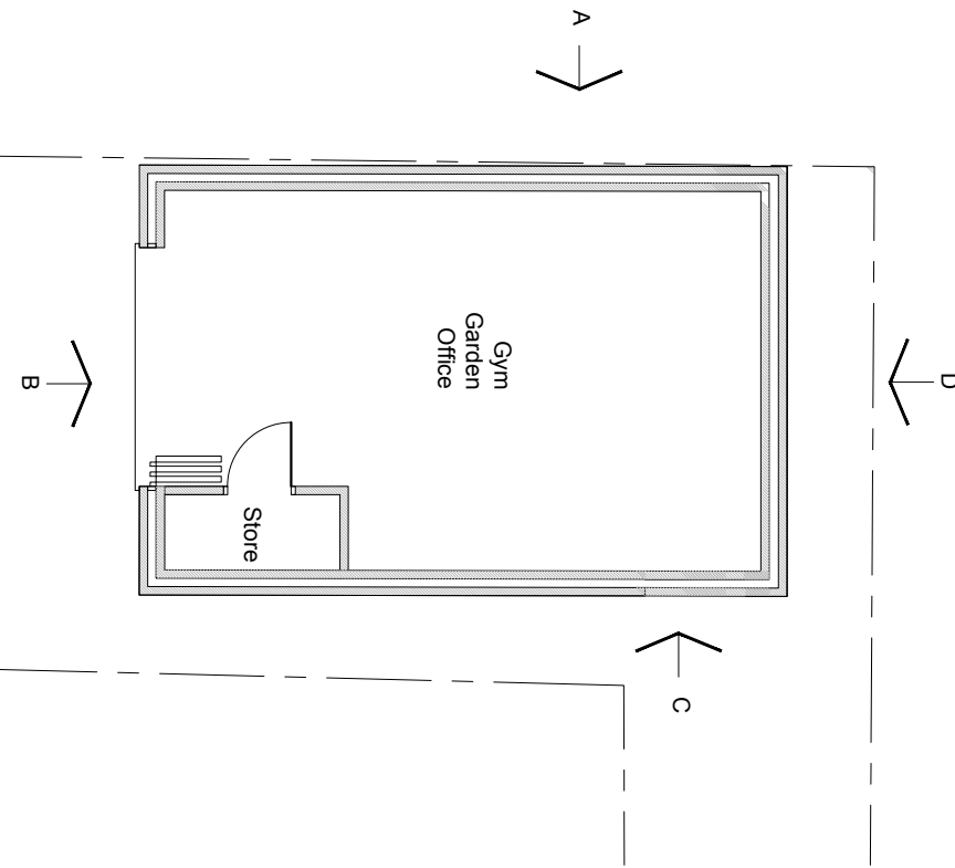
Proposed Plan (1:100)
