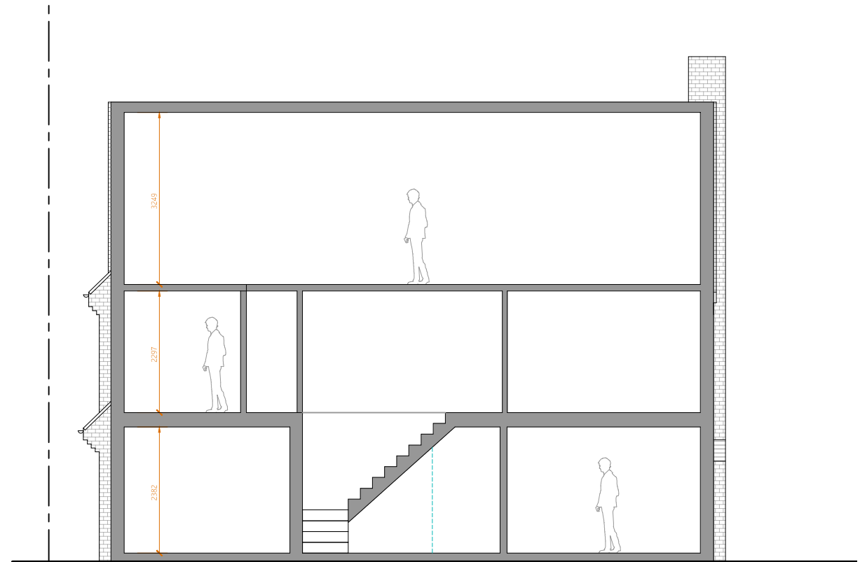
10 Proposed Front Section SCALE: 1/100
