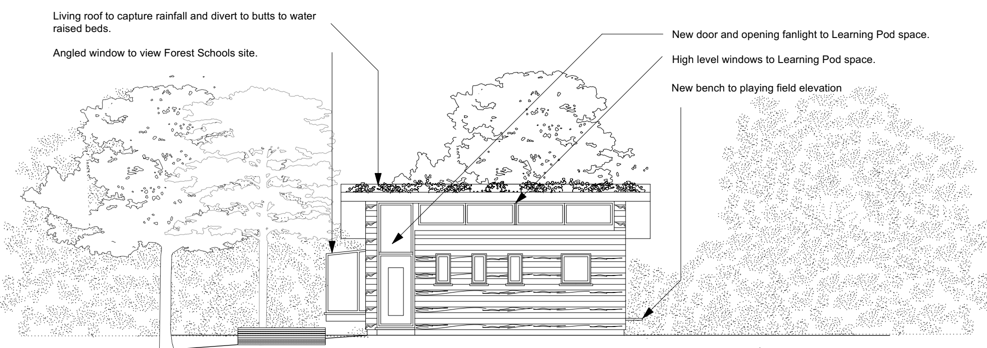
Proposed Elevation facing boundary
