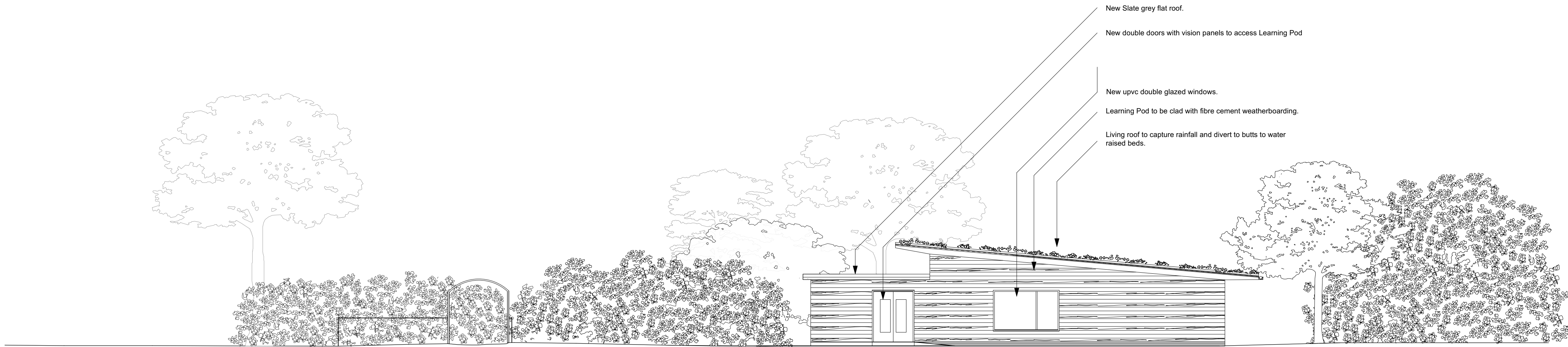
Proposed Elevation facing the Playing Field
