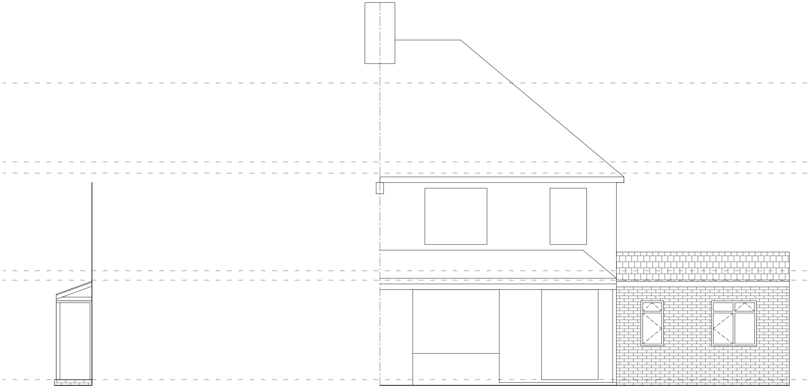
PROPOSED FLANK ELEVATION
