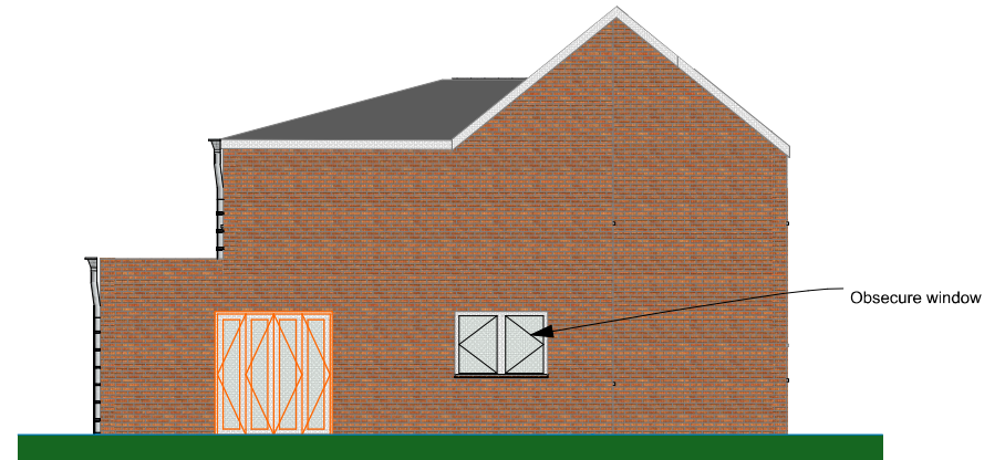
Proposed Left Side Elevation 1:100
