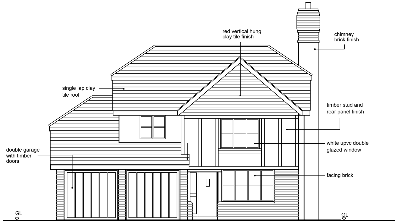
FRONT ELEVATION
