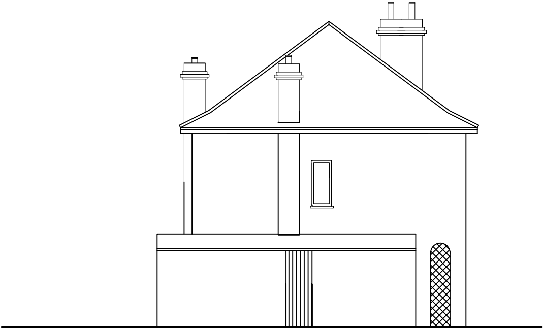
EXISTING SIDE ELEVATION 1
