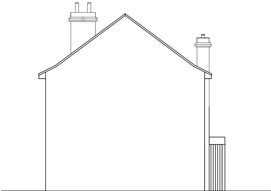
EXISTING SIDE ELEVATION 2
