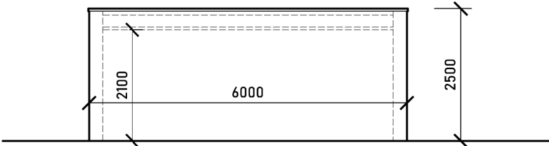
PROPOSED OUTBUILDING SIDE ELEVATION
