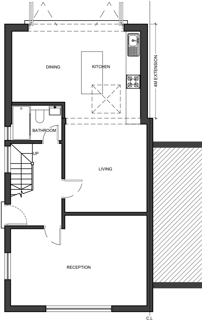
01 - GROUND FLOOR PLAN
