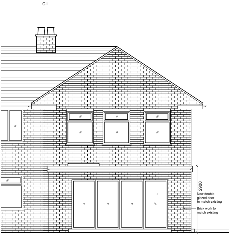
03 - REAR ELEVATION
