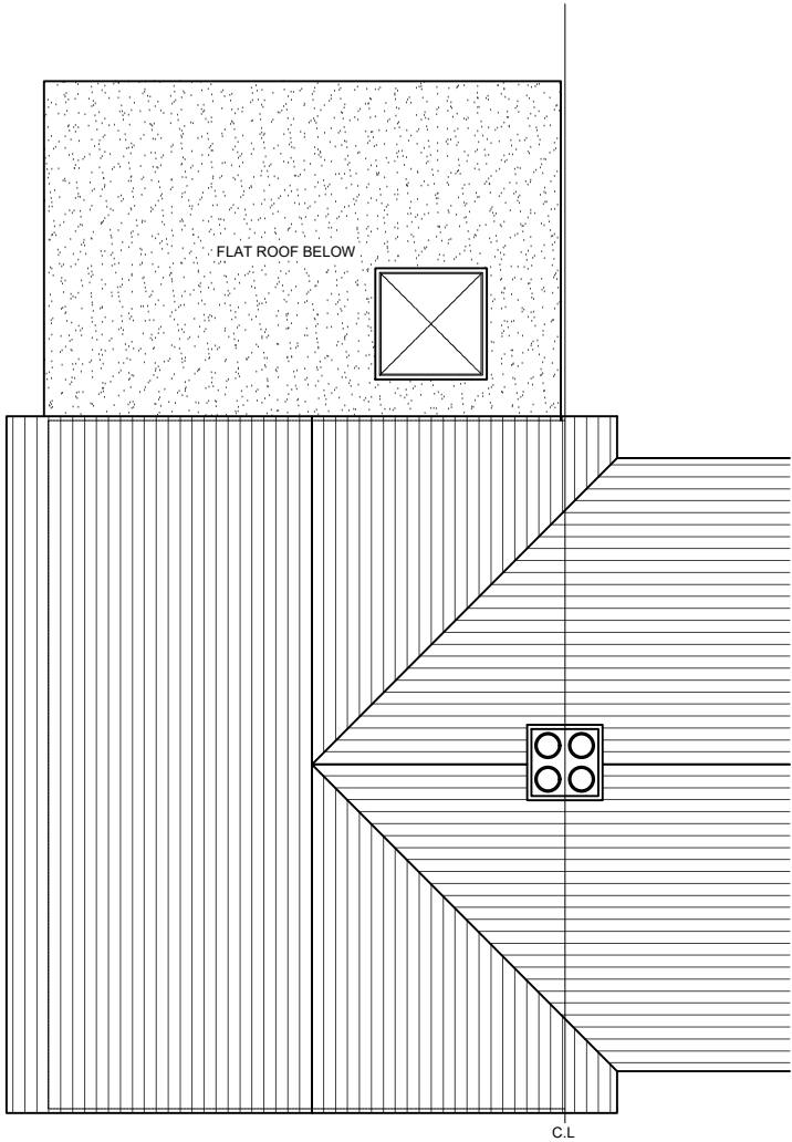
02 - ROOF PLAN
