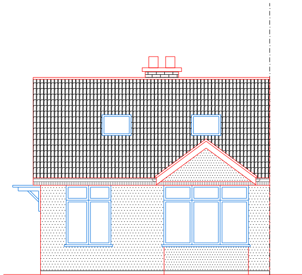
PROPOSED FRONT ELEVATION (NO CHANGE)
