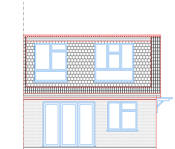
PROPOSED REAR ELEVATION (NO CHANGE)
