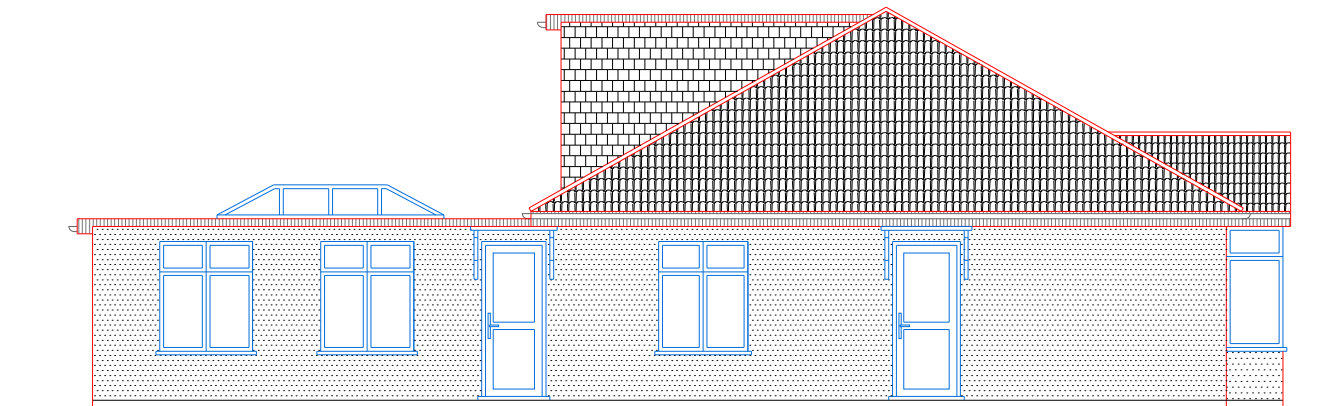
PROPOSED SIDE ELEVATION-2 (NO CHANGE)
