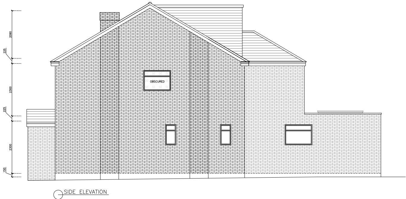
SIDE ELEVATION
