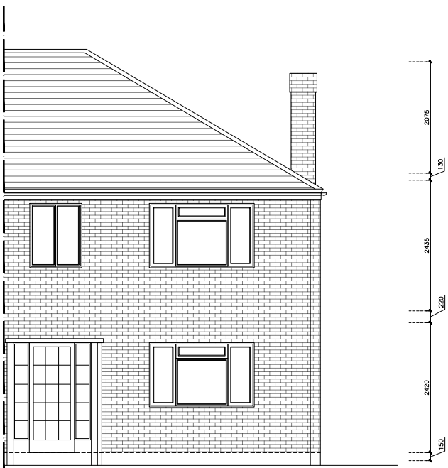
FRONT ELEVATION
