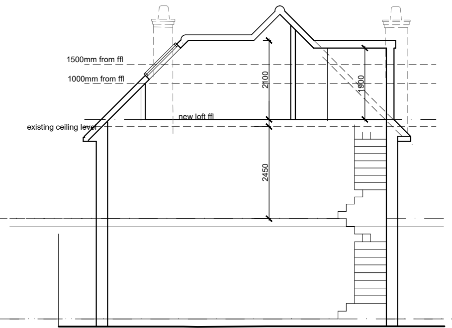
CROSS SECTION
