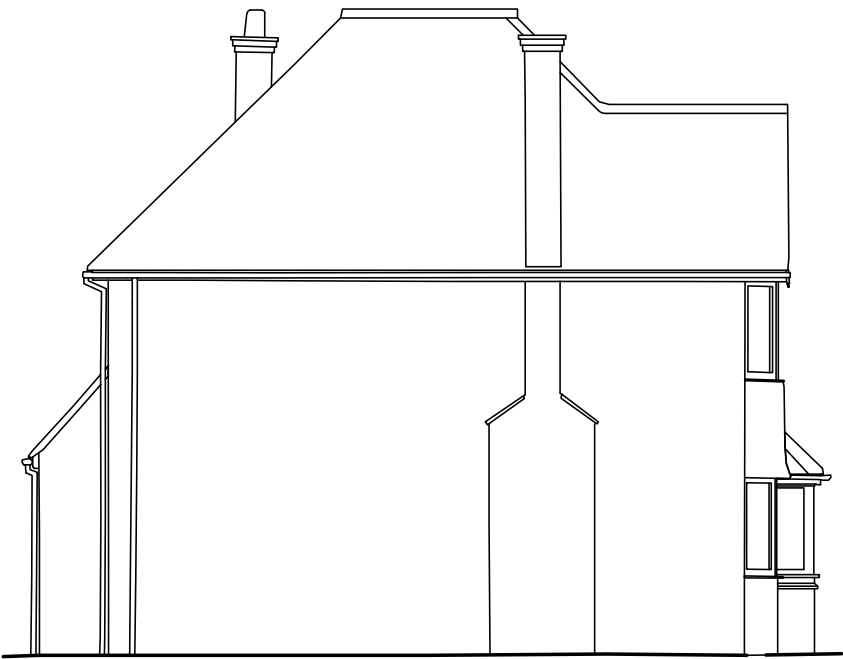
NORTH ELEVATION
