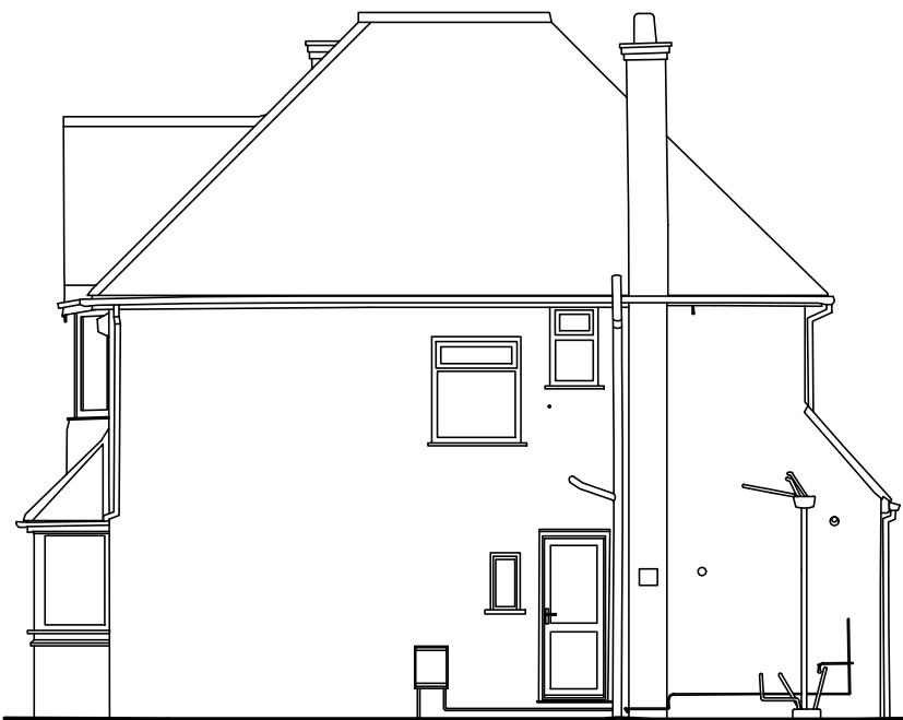
SOUTH ELEVATION
