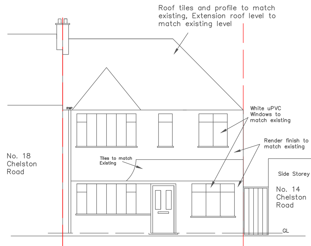
PROPOSED FRONT VIEW
