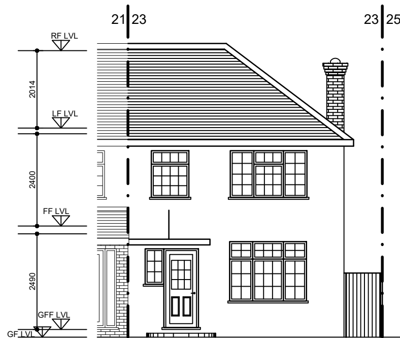
FRONT ELEVATION APPROVED
