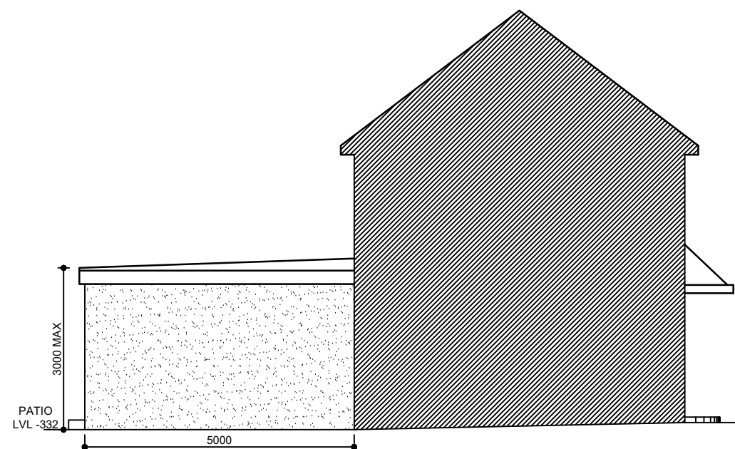
SIDE ELEVATION APPROVED (AS VIEWED FROM NO.21)
