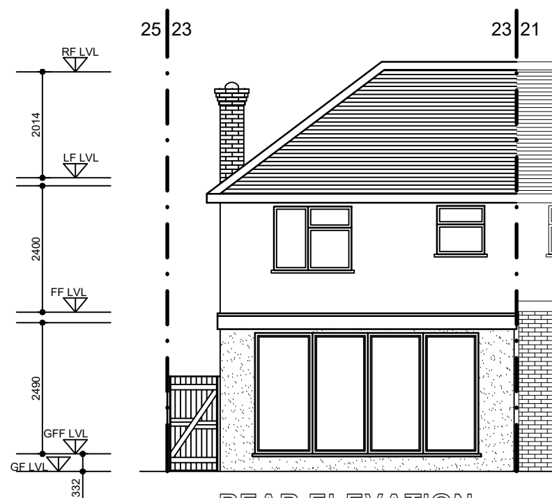
REAR ELEVATION APPROVED
