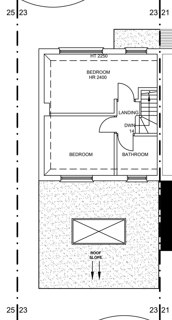
APPROVED FIRST FLOOR PLAN
