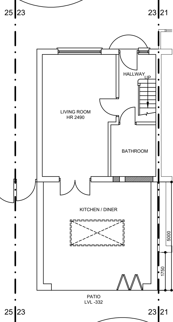
APPROVED GROUND FLOOR PLAN (REF : 76944/APP/2021/4586)
