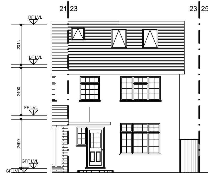
FRONT ELEVATION EXISTING
