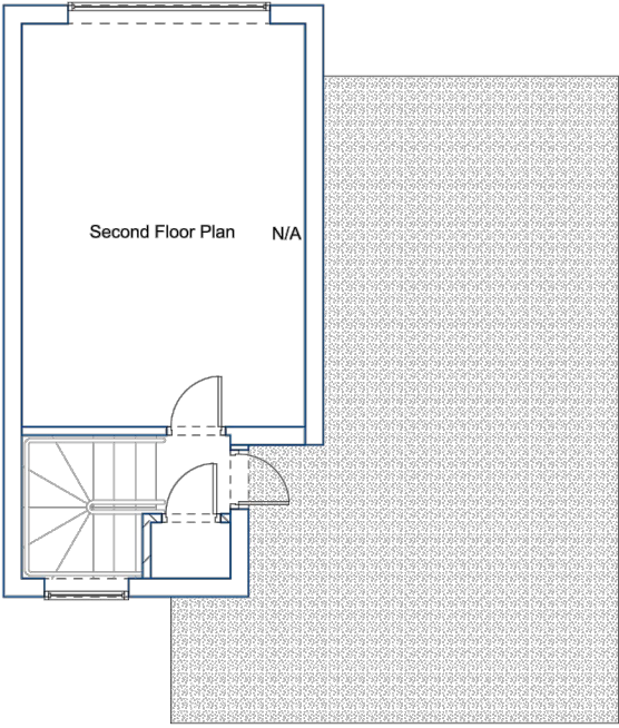
Existing Second Floor Plan
