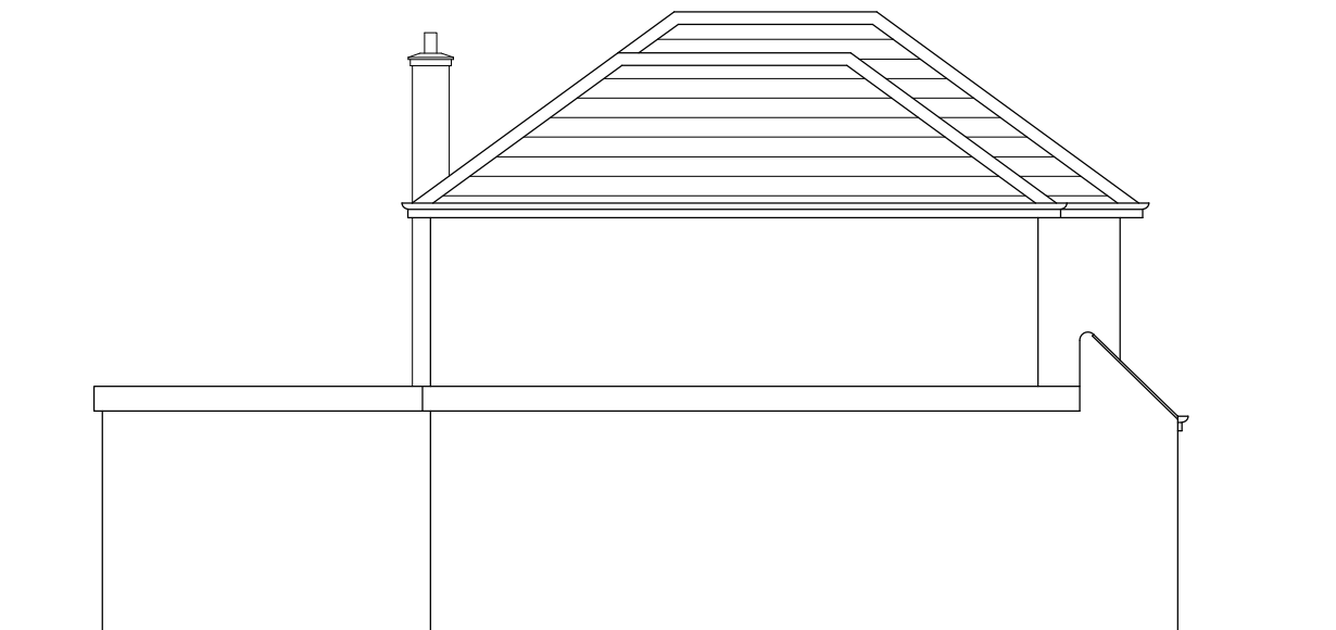
PRE-EXISTING SIDE (EAST) ELEVATION
