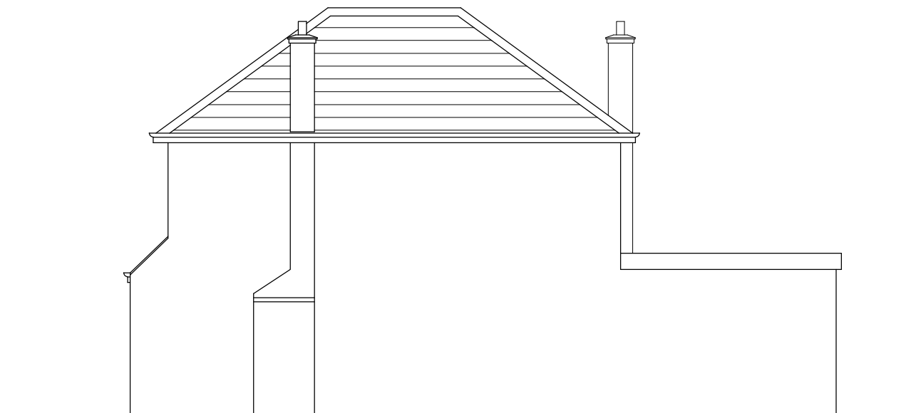
PRE-EXISTING SIDE (WEST) ELEVATION
