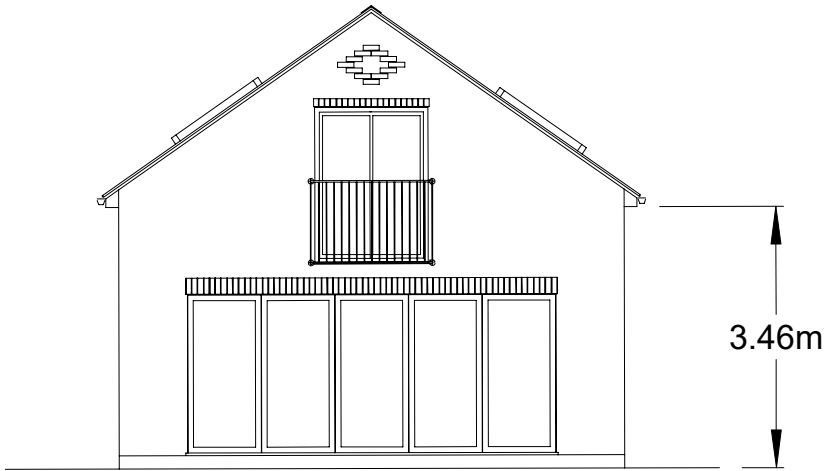
SOUTH ELEVATION
