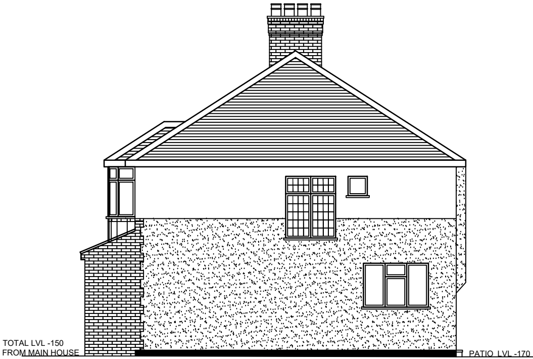
SIDE ELEVATION EXISTING (AS VIEWED FROM NO.12)
