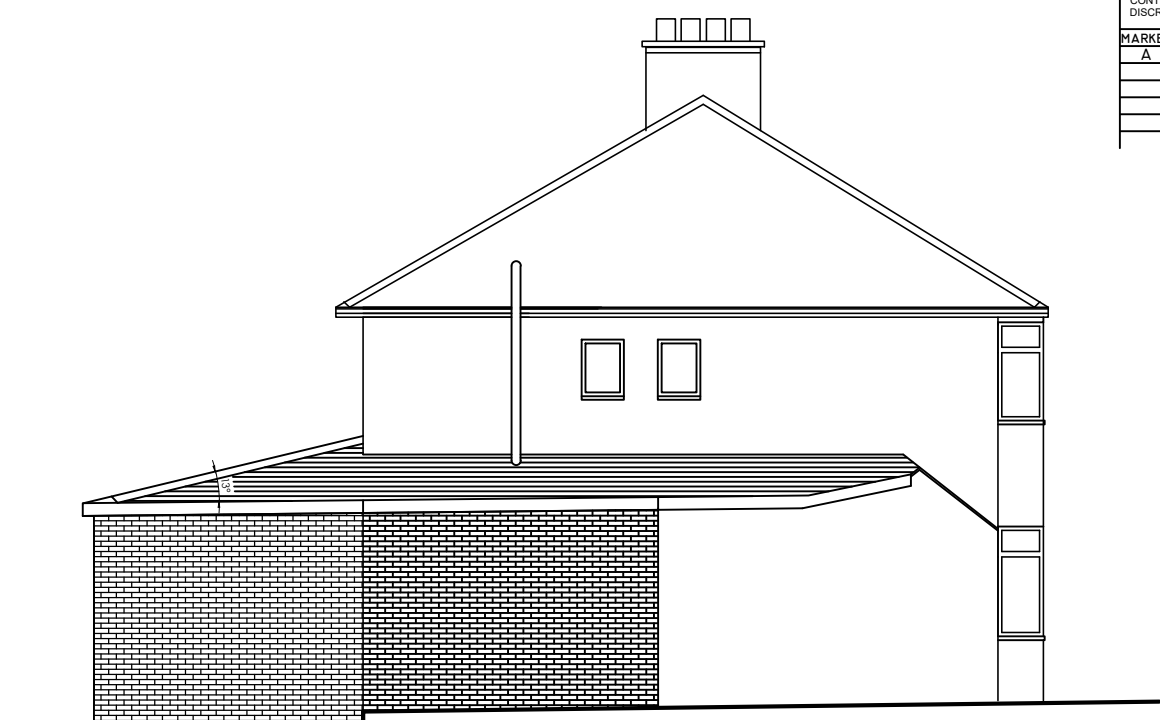
PROP SIDE ELEVATION
