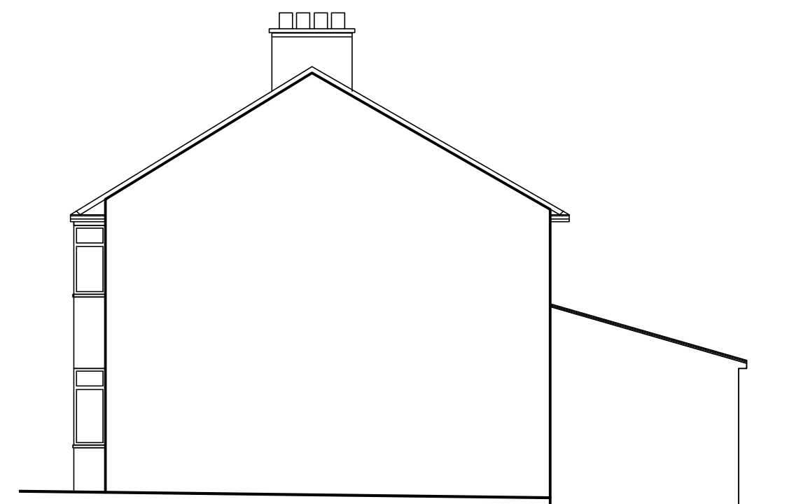
EXTG OTHER SIDE ELEVATION
