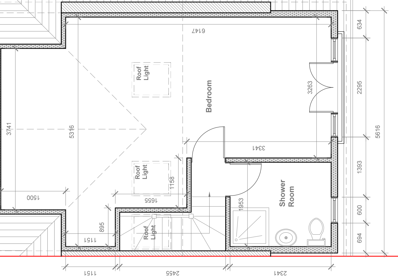
Proposed Loft Plan Scale 1:50
