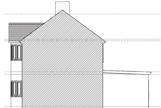
PROPOSED SIDE (1:100)
