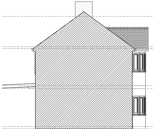
PROPOSED SIDE (1:100)
