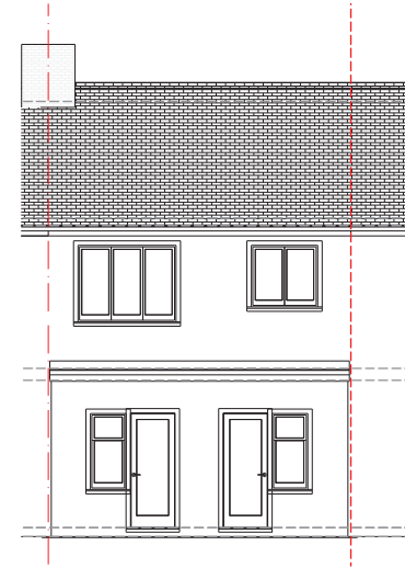
PROPOSED REAR (1:100)
