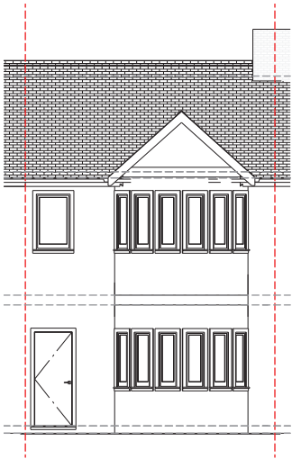
PROPOSED FRONT (1:100)
