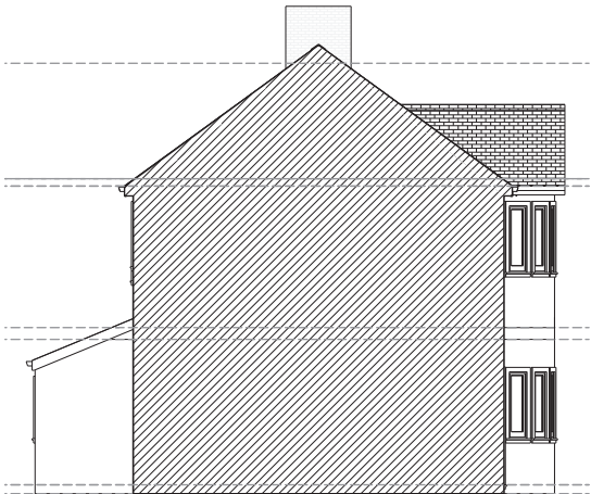
EXISTING SIDE (1:100)
