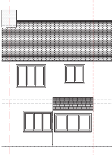
EXISTING REAR (1:100)
