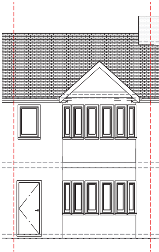
EXISTING FRONT (1:100)
