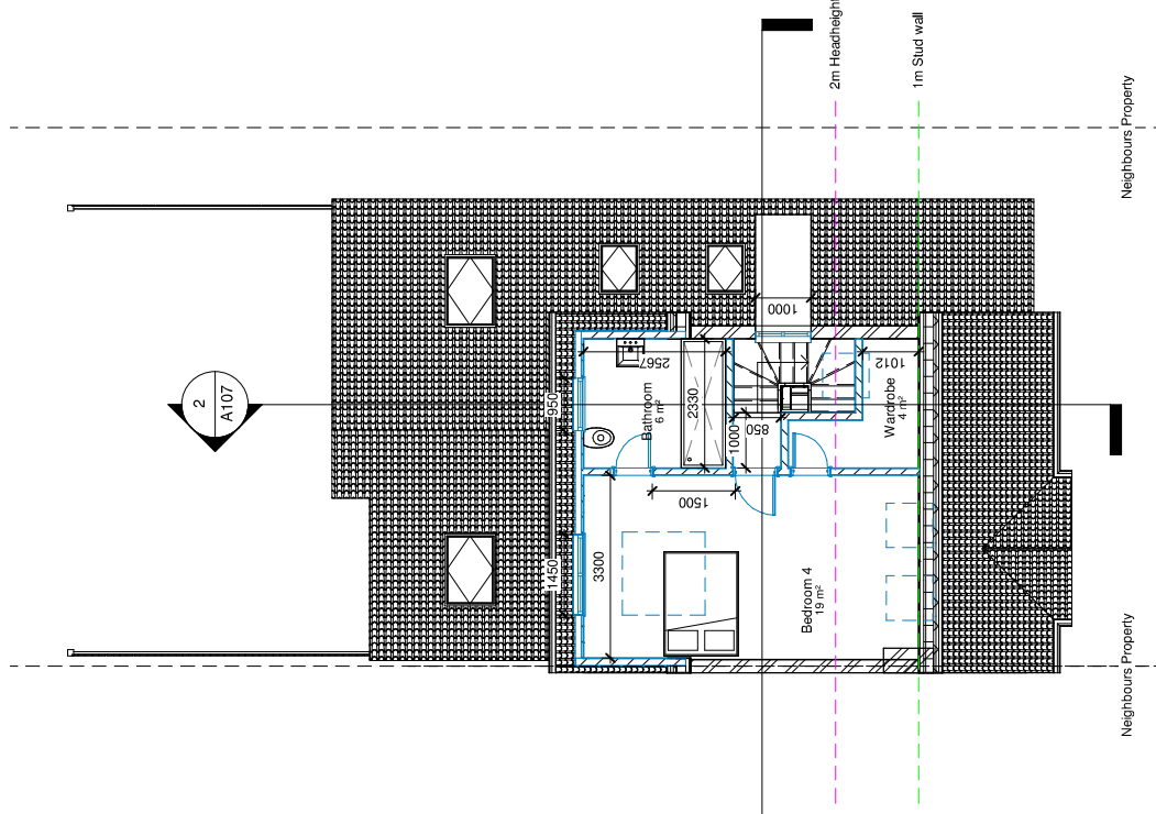
2 Loft - Proposed 1 : 100
