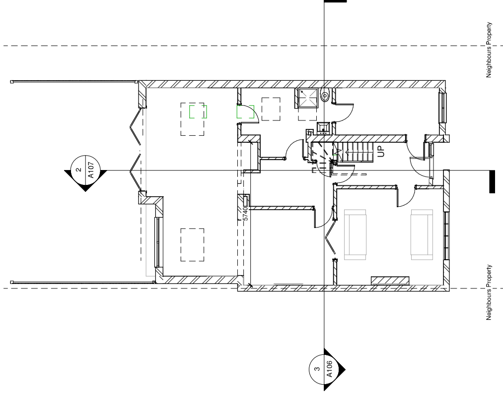
2 00 - Proposed 1 : 100
