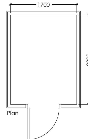
Cycle Shed Details 1 : 50
