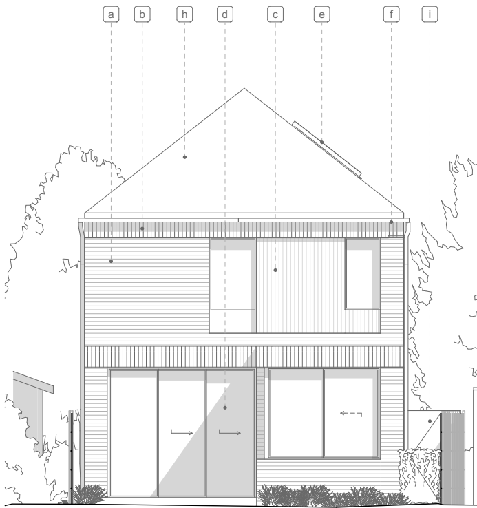
1:100 Proposed East Elevation
