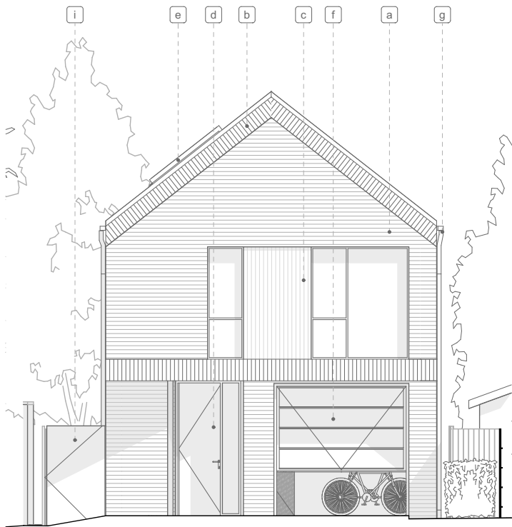
1:100 Proposed West Elevation
