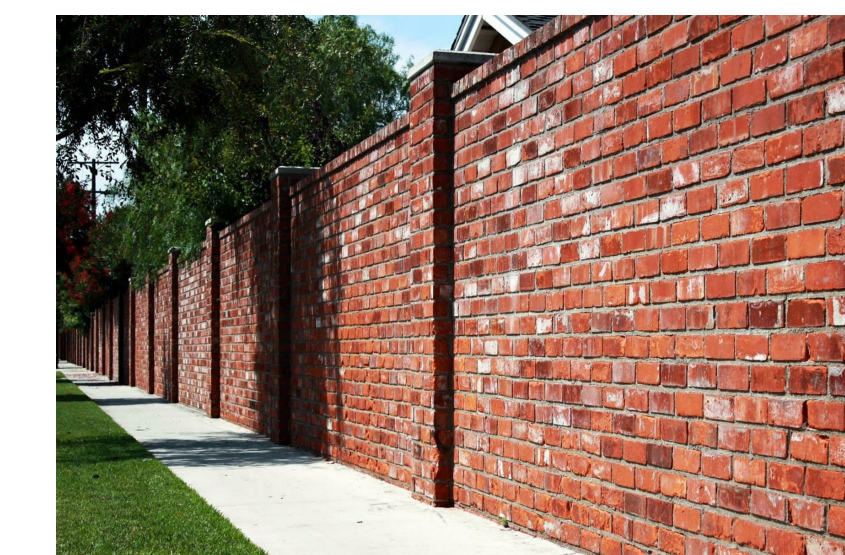
Red Brick perimeter wall where level differs, up to 1.2m
