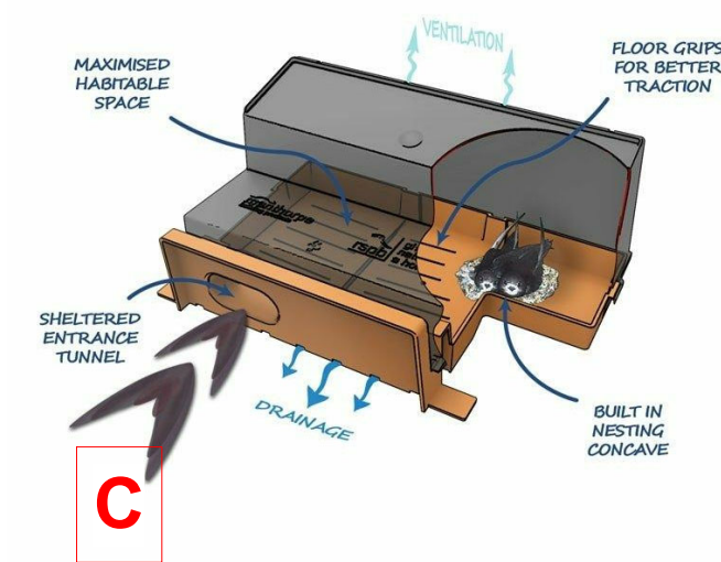
Manthorpe Swift Brick nest integrated within the brick wall
