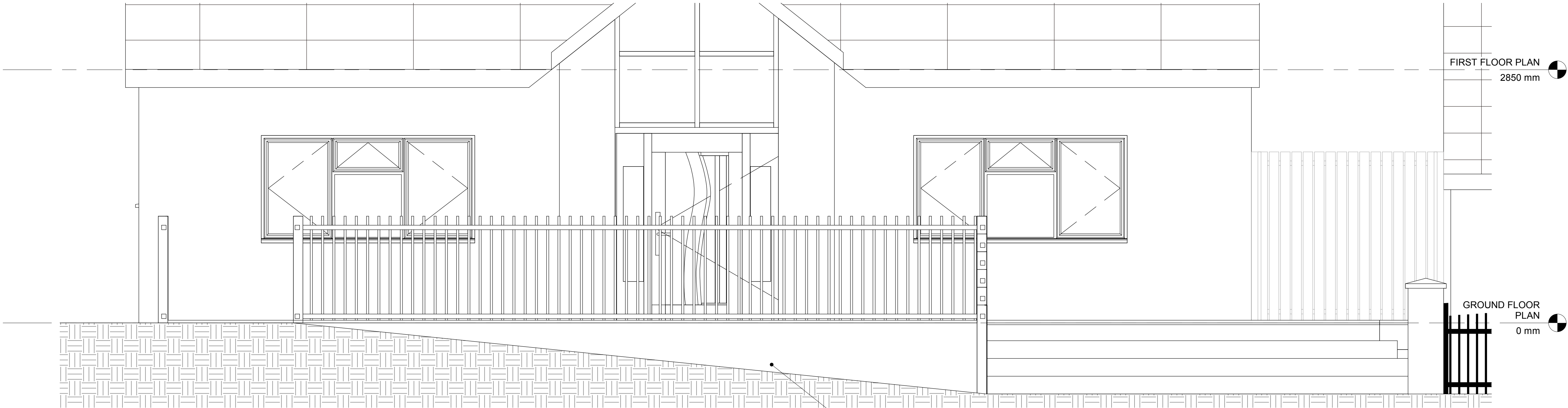
1 Entrance Ramp 1 : 25
