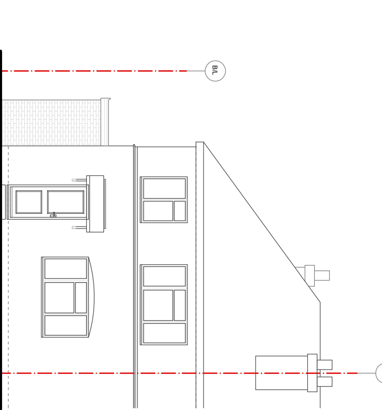
FRONT ELEVATION AS PROPOSED
