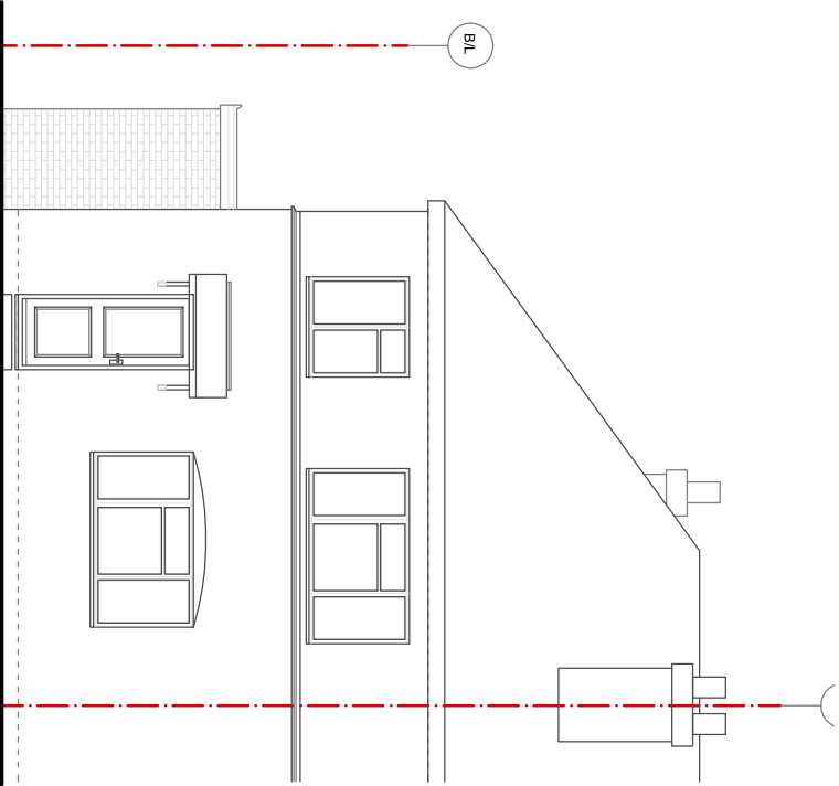
FRONT ELEVATION AS PROPOSED
