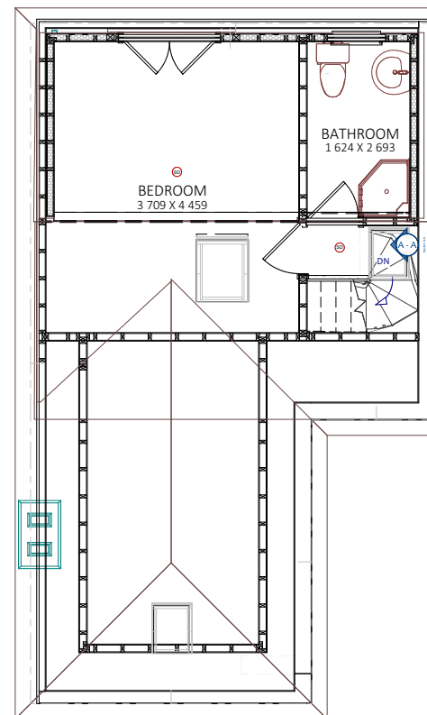
Proposed Upper Floor Pln
