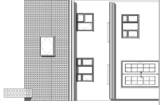
Rear elevation - Proposed 1 : 100
