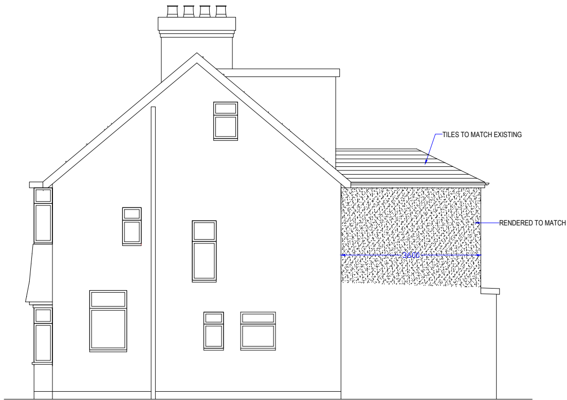
PROPOSED RIGHT ELEVATION
