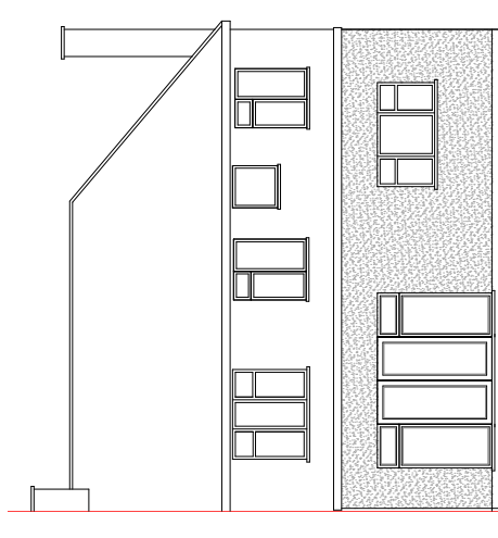
PROPOSED REAR ELEVATION 1:100
