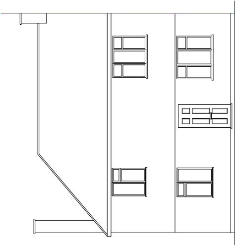
EXISTING FRONT ELEVATION 1:100
