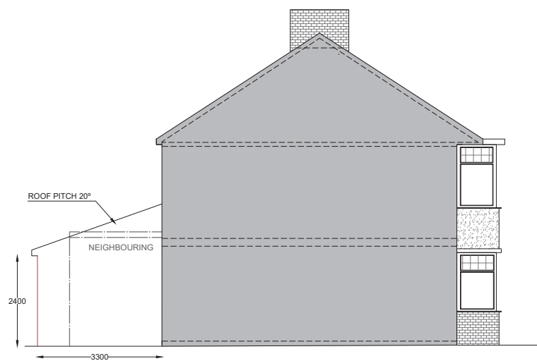
PROPOSED LEFT SIDE ELEVATION
