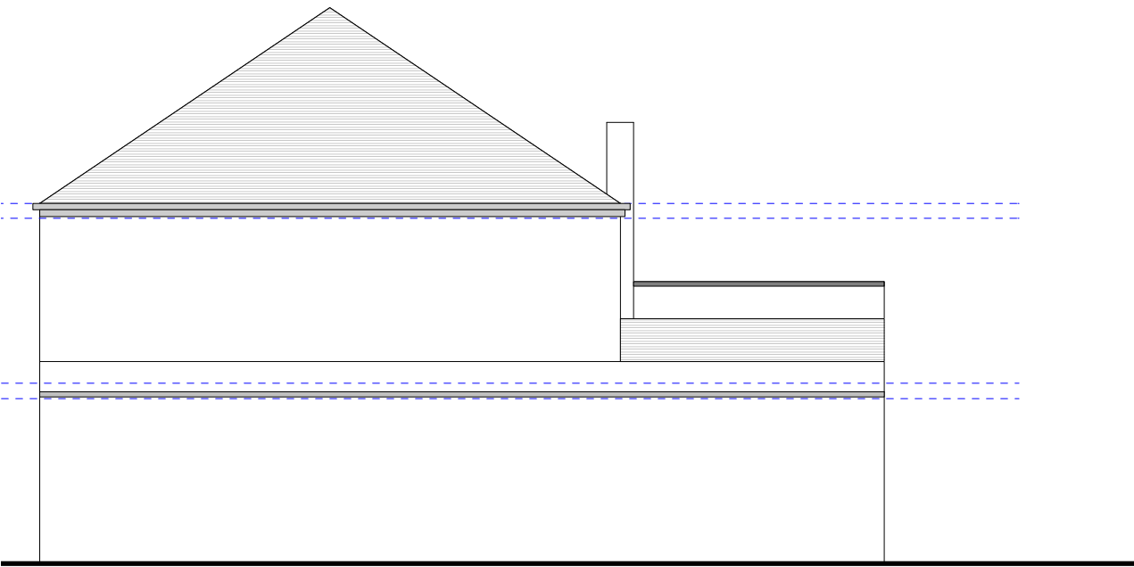
1 EX-10 SIDE ELEVATION PLAN Scale: 1/100
