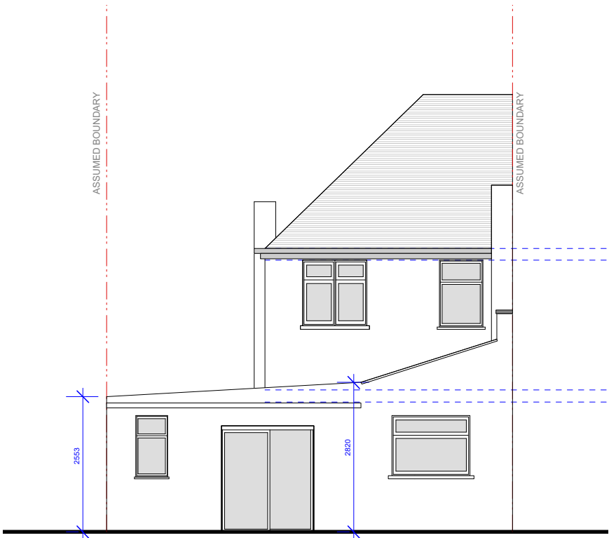
1 EX-10 REAR ELEVATION PLAN Scale: 1/100
