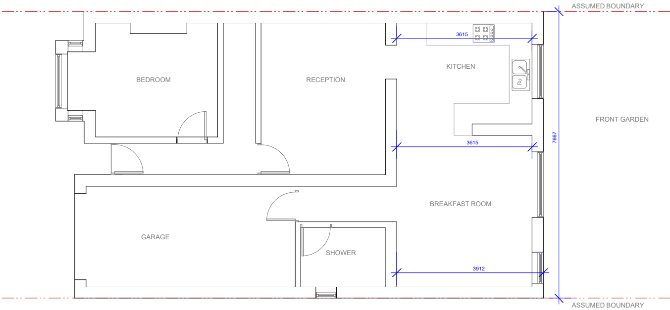
1 EX-10 GROUND FLOOR PLAN Scale: 1/100
