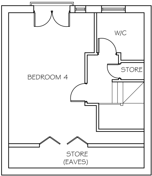
EXISTING ATTIC FLOOR PLAN
