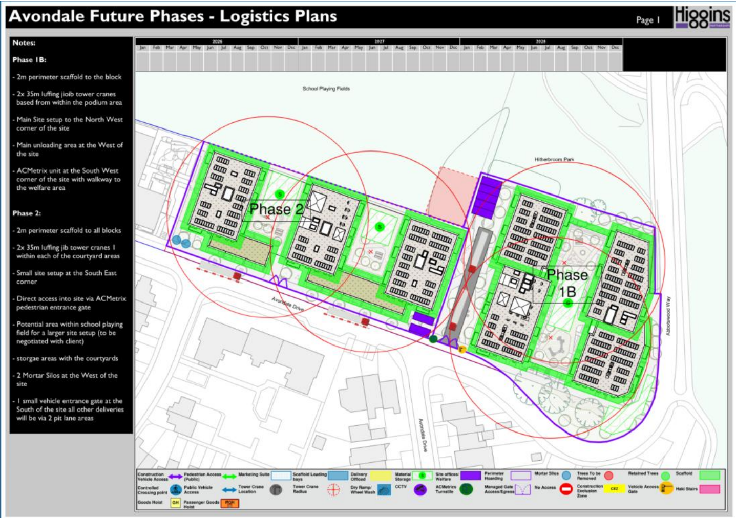
FIGURE 15: Site Boundary Phase Logistical Plan –
