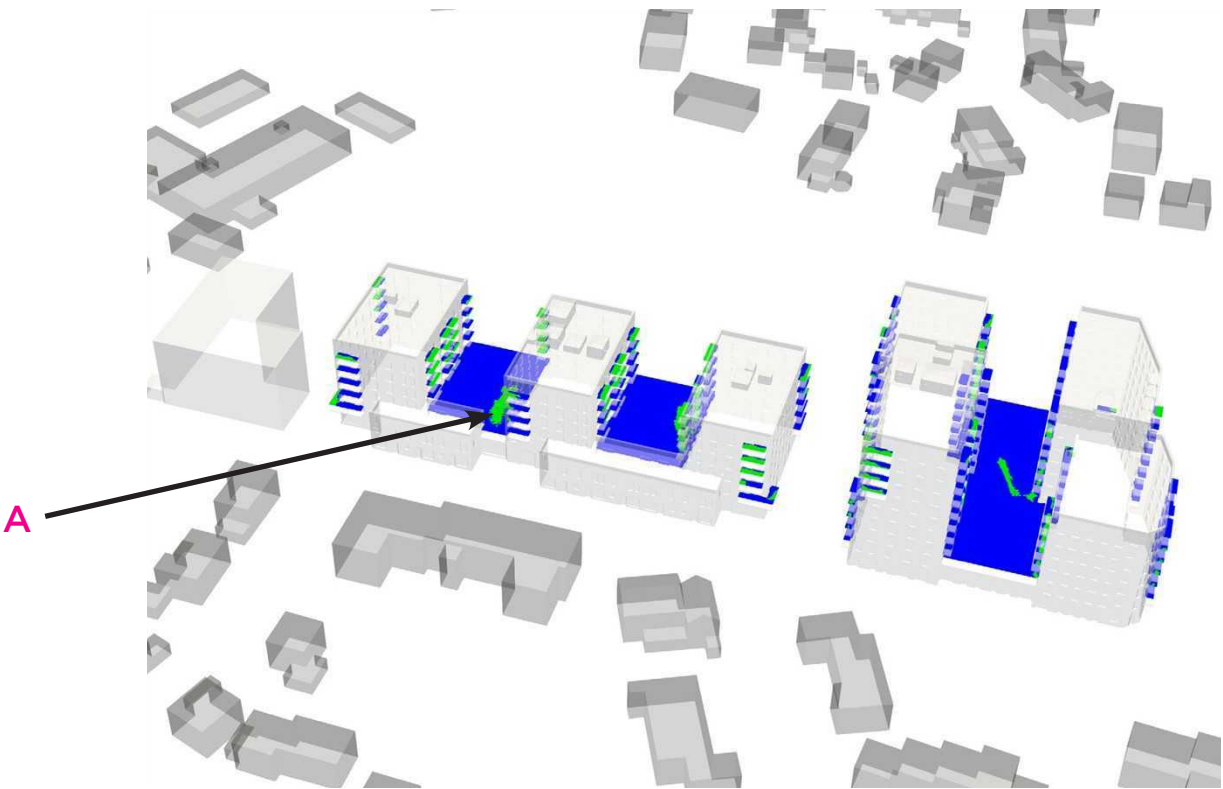
Figure 12. Lawson Comfort Contours, Proposed Site with Existing Surrounds and Mitigations, Summer Condition, Southern Aspect
