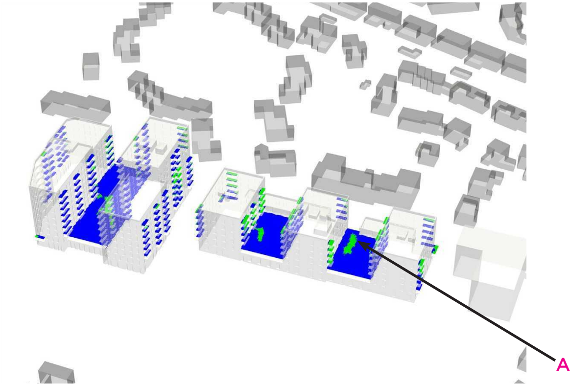
Figure 10. Lawson Comfort Contours, Proposed Site with Existing Surrounds and Mitigations, Summer Condition, Northern Aspect
