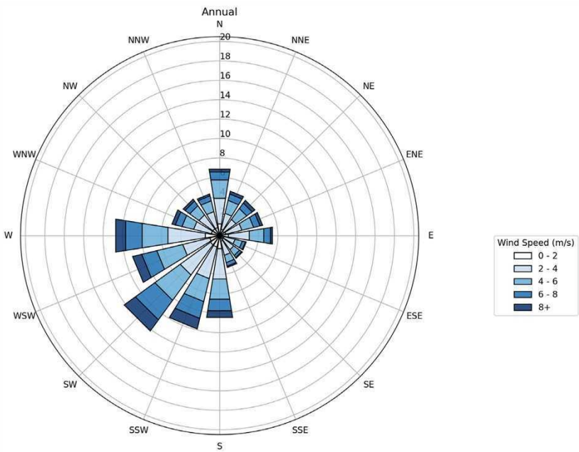
Figure 7. Wind Speeds and Frequencies of Occurrence for the London Region (corrected to open terrain at 10m)
