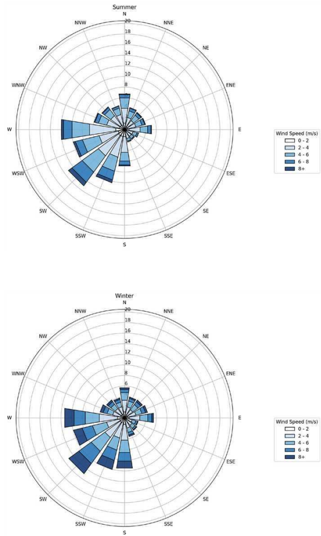
Figure 8. Summer (top) and Winter (bottom) Wind Speeds and Frequencies of Occurrence for the London Region (corrected to open terrain at 10m)
