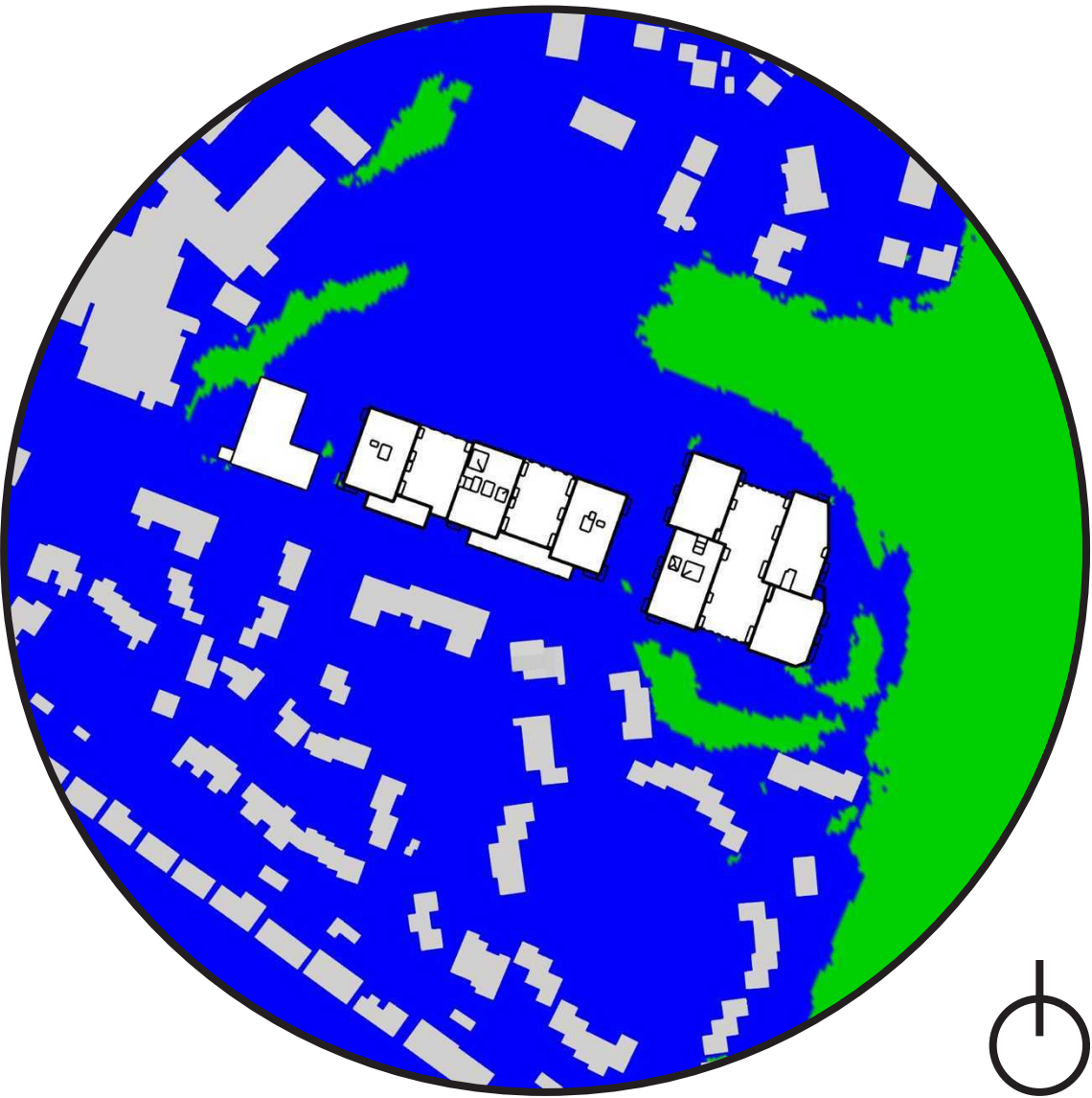
Figure 1. Lawson Comfort Contours, Proposed Site with Existing Surrounds and Mitigations, Summer Condition
