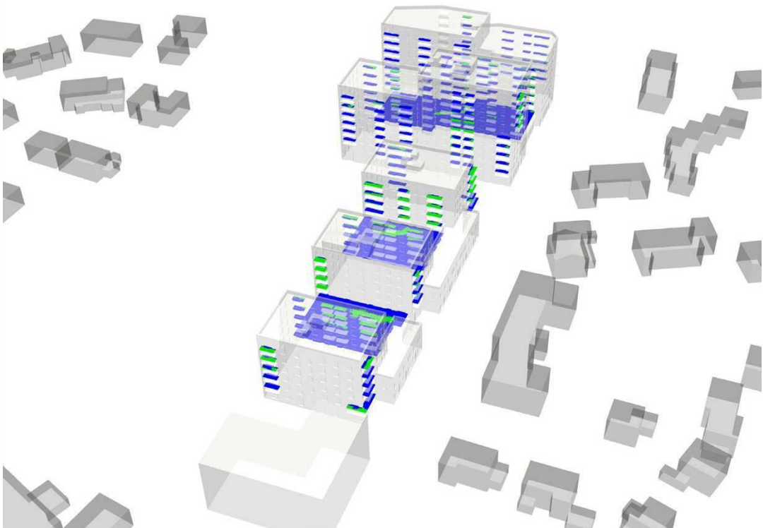
Figure 13. Lawson Comfort Contours, Proposed Site with Existing Surrounds and Mitigations, Summer Condition, Western Aspect
