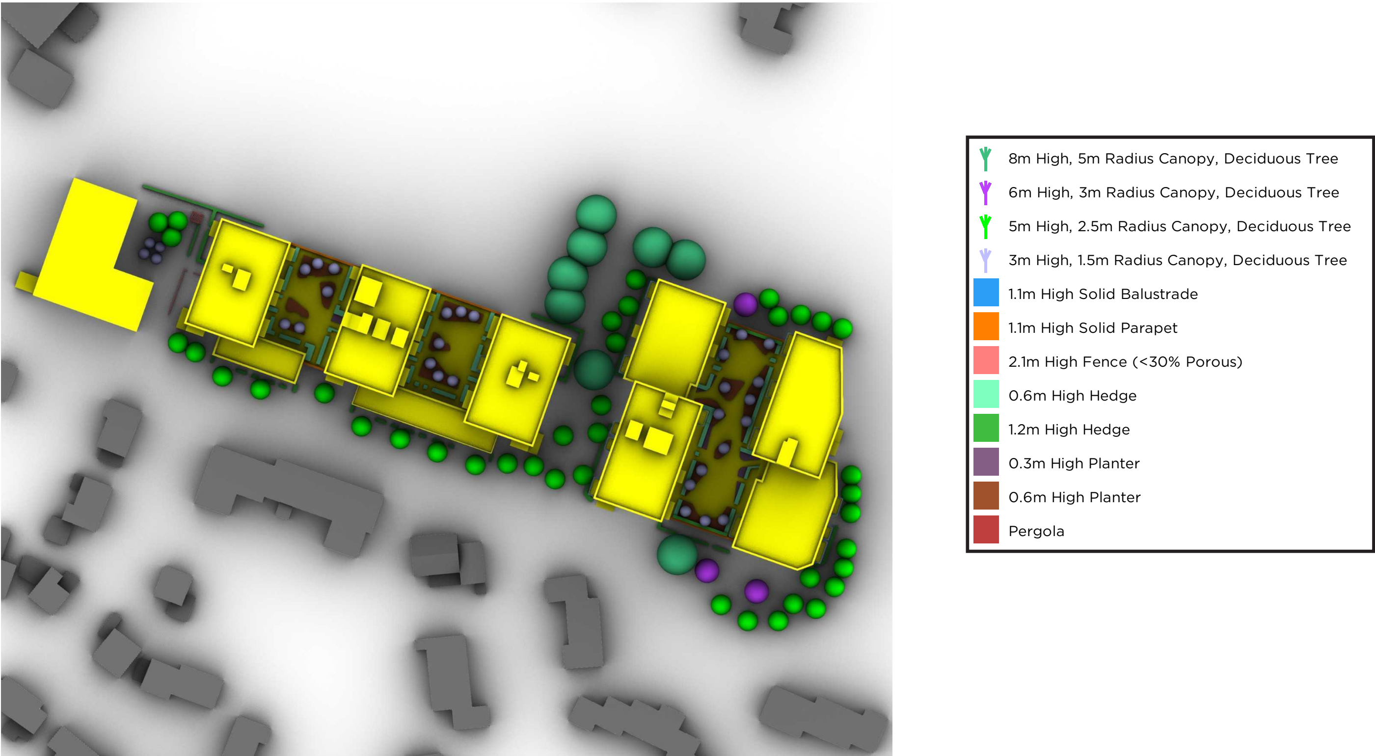
Figure D.1. Tested Mitigation Render - Plan View
