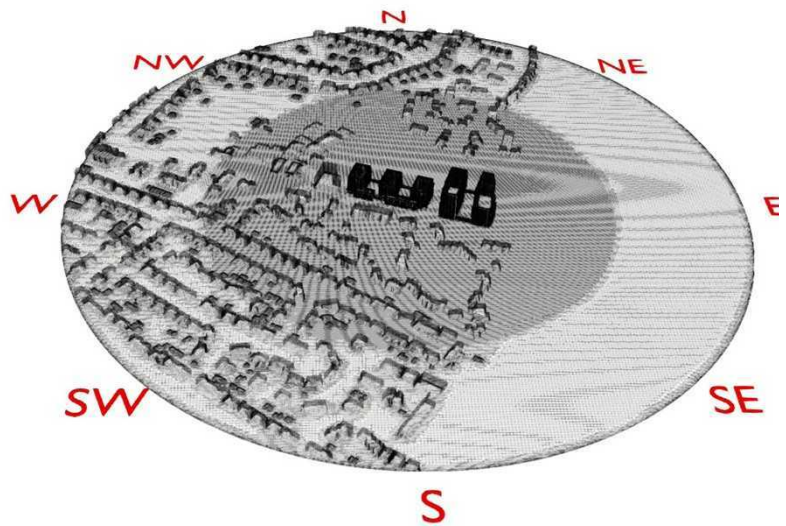
Figure 6. Computational Grid (Proposed Site with Existing Surrounds)
