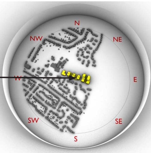
Figure 5. Computational Domain (Proposed Site with Existing Surrounds)
