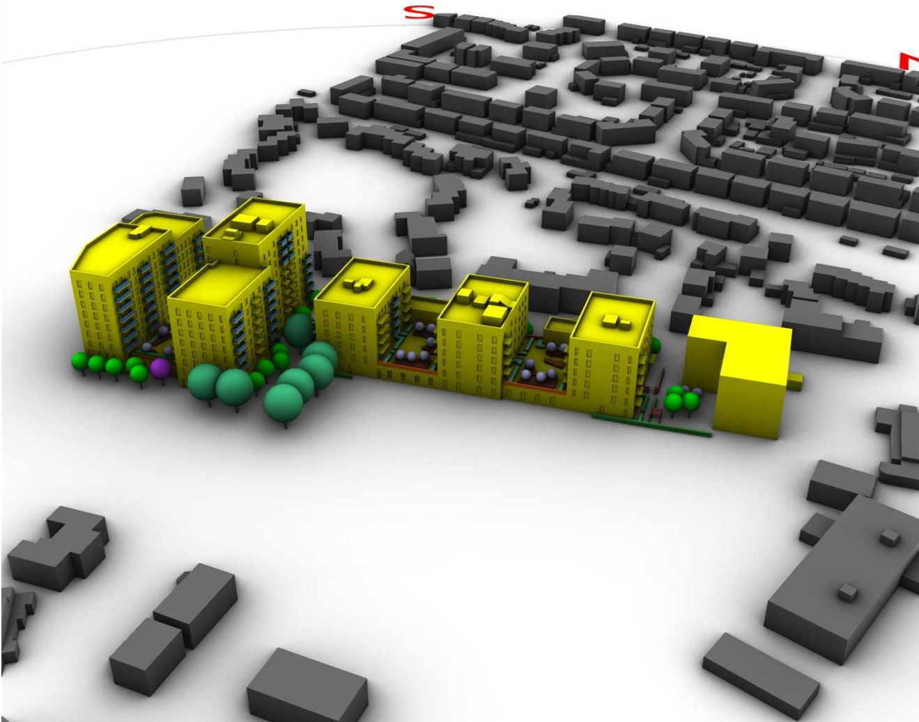
Figure D.2. Tested Mitigation Render - Northern Aspect
