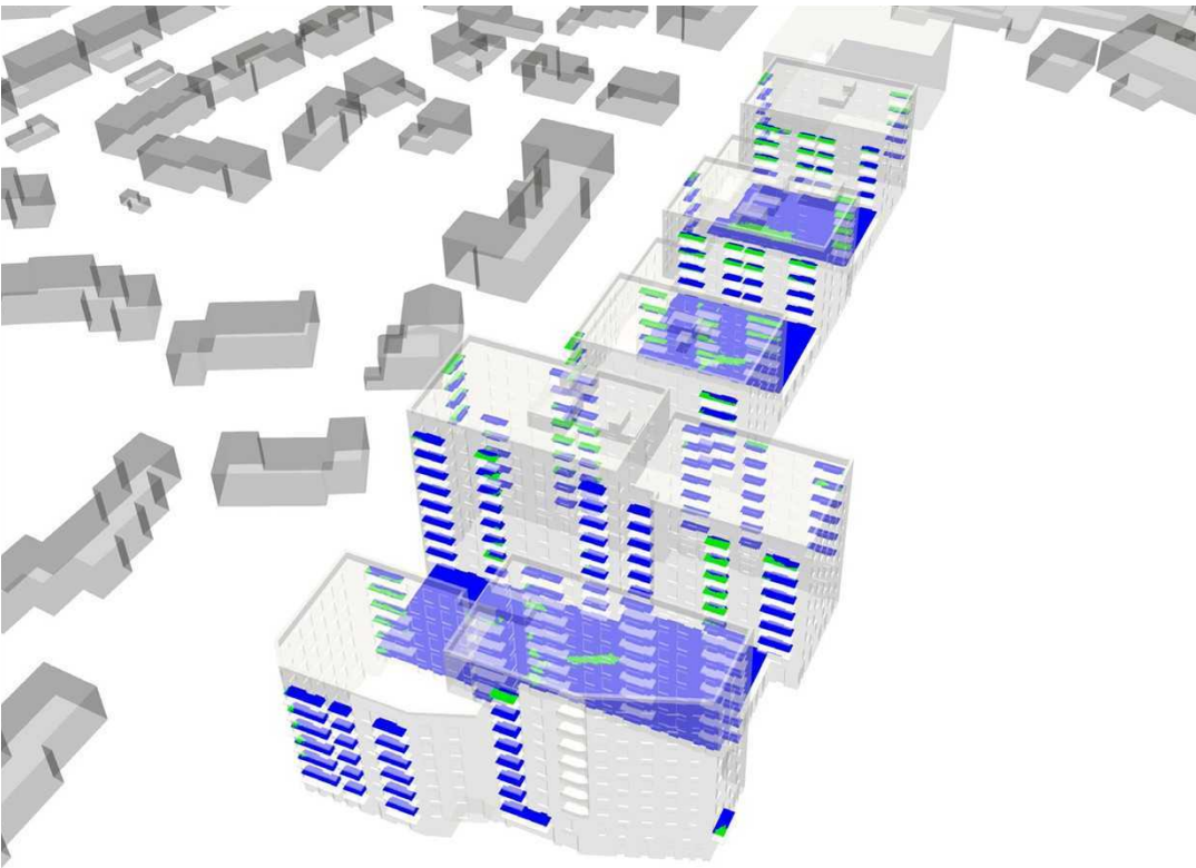
Figure 11. Lawson Comfort Contours, Proposed Site with Existing Surrounds and Mitigations, Summer Condition, Eastern Aspect
