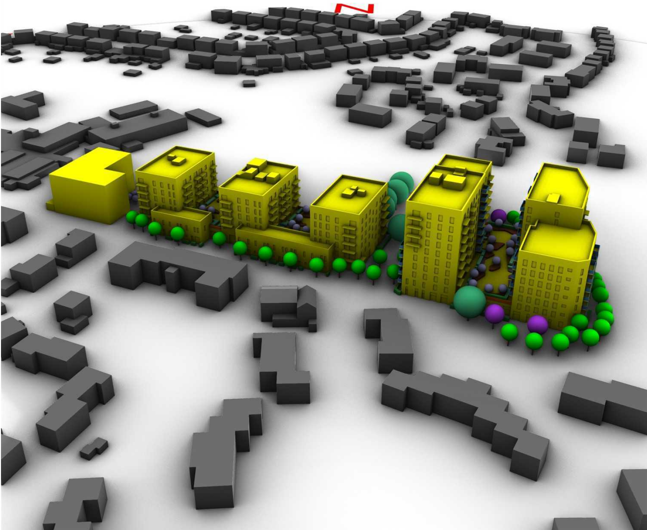
Figure D.4. Tested Mitigation Render - Southern Aspect
