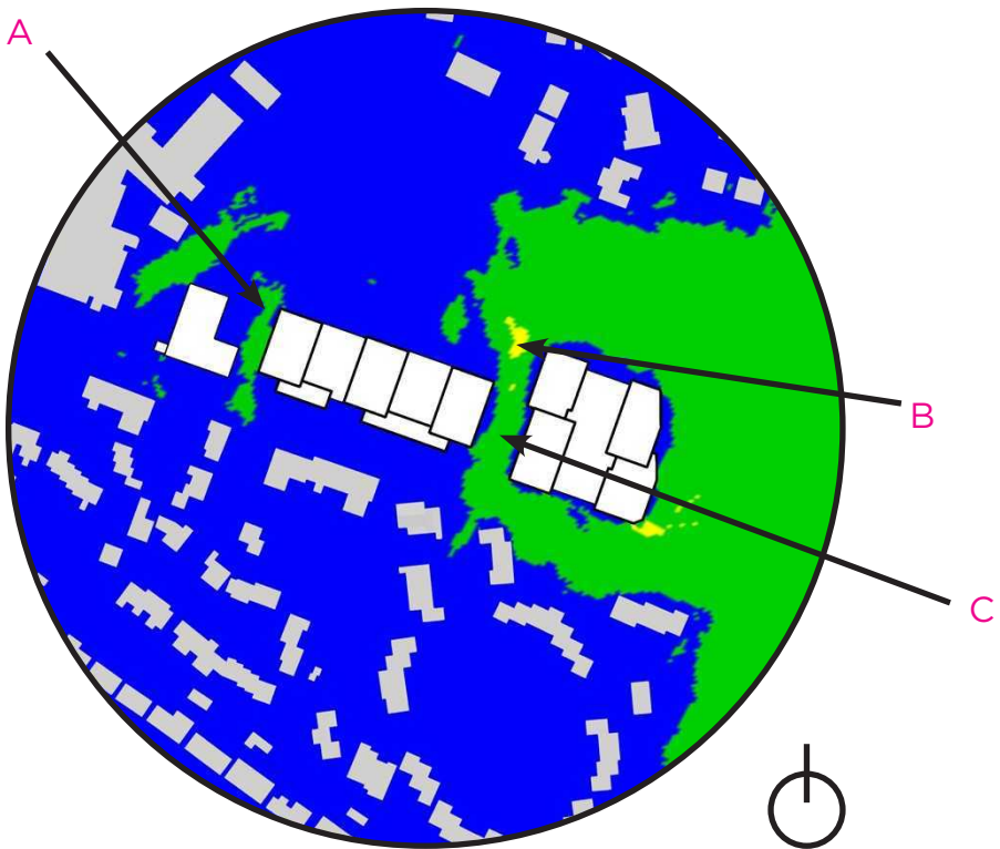
Figure 19. Lawson Comfort Contours, Proposed Site with Existing Surrounds, Summer Condition
