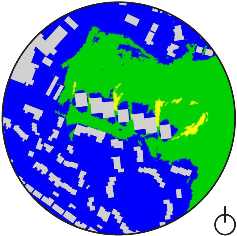
Figure 18. Lawson Comfort Contours, Existing Site with Existing Surrounds, Summer Condition
