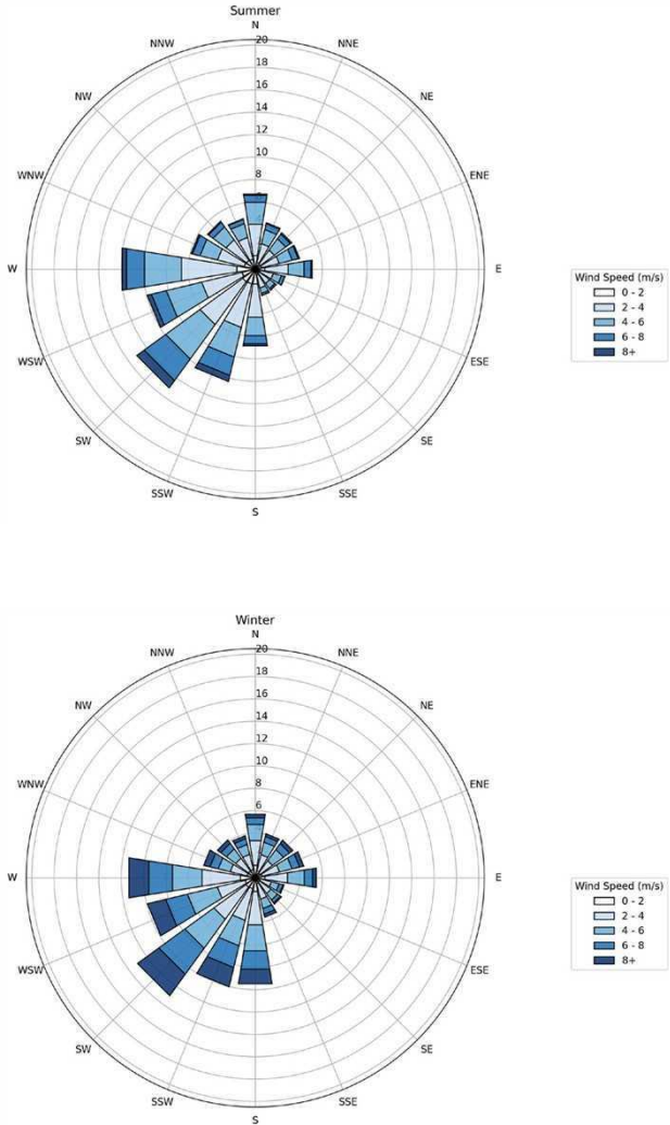
Figure 11. Summer (top) and Winter (bottom) Wind Speeds and Frequencies of Occurrence for the London Region (corrected to open terrain at 10m)
