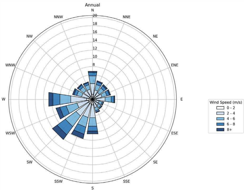
Figure 10. Wind Speeds and Frequencies of Occurrence for the London Region (corrected to open terrain at 10m)
