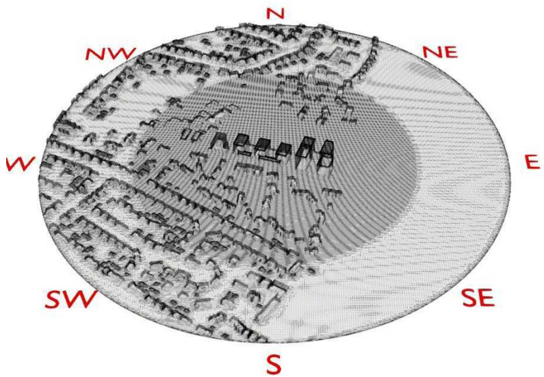
Figure 9. Computational Grid (Proposed Site with Existing Surrounds)
