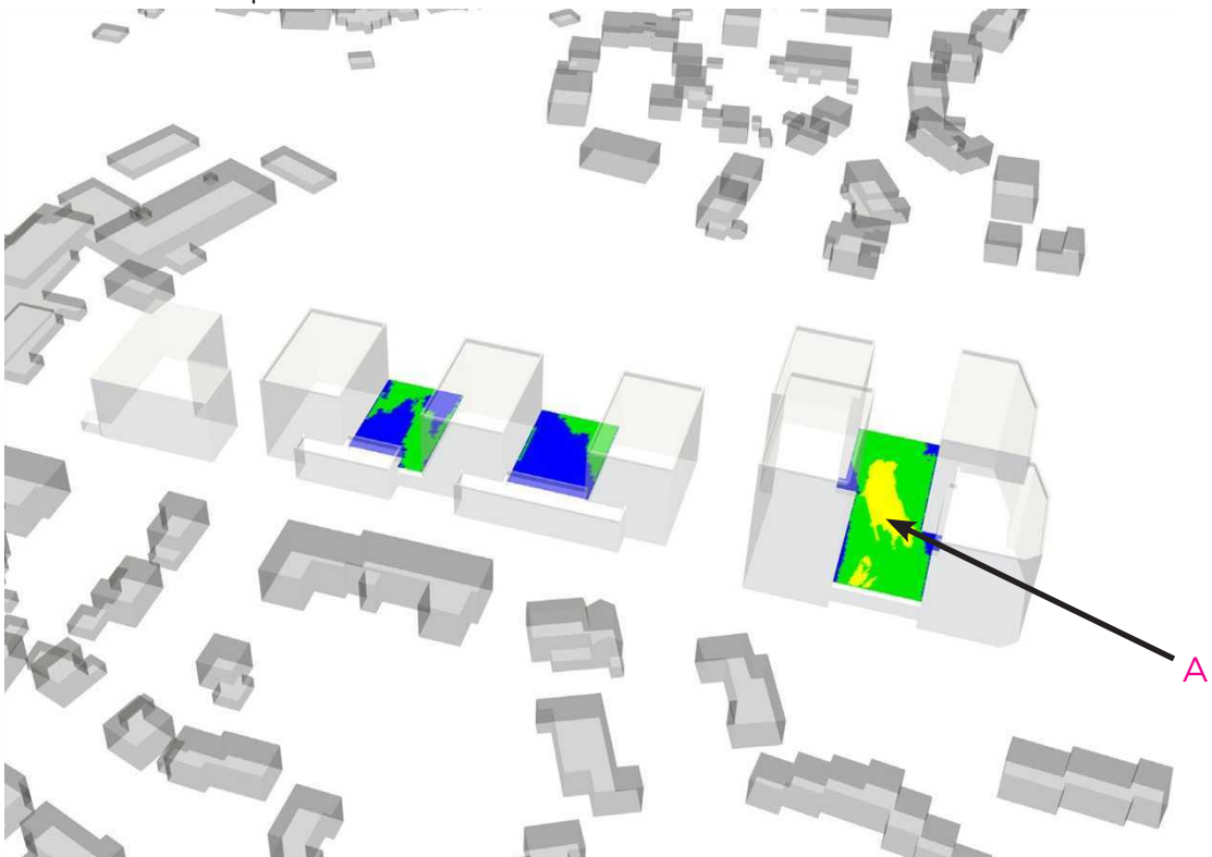
Figure 21. Lawson Comfort Contours, Proposed Site with Existing Surrounds, Summer Condition, Southern Aspect
