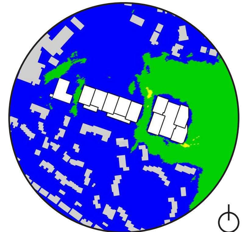
Figure 4. Lawson Comfort Contours, Proposed Site with Existing Surrounds, Summer Condition
