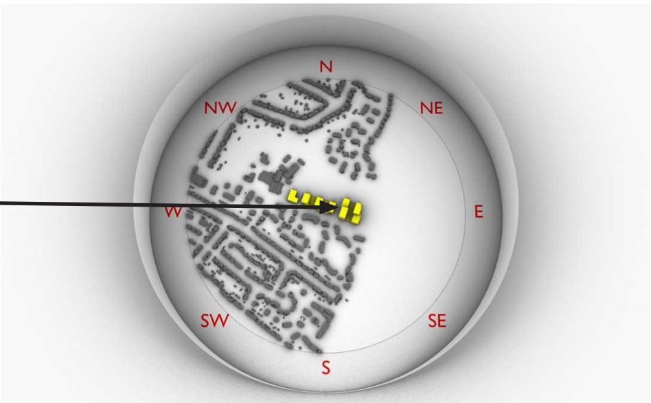
Figure 8. Computational Domain (Proposed Site with Existing Surrounds)
