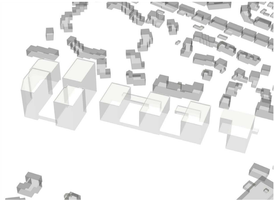
Figure 14. Lawson Safety Contours, Proposed Site with Existing Surrounds, Annual Condition, Northern Aspect
