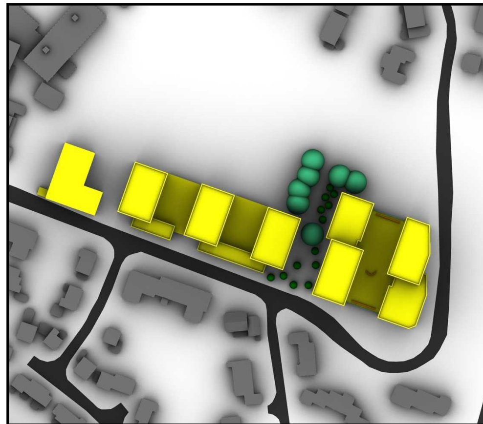
Figure 22. Recommended Mitigation Treatments, Plan View
