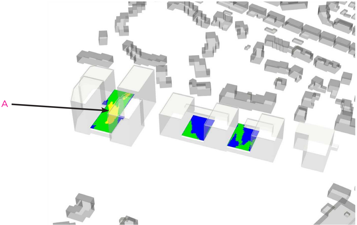
Figure 20. Lawson Comfort Contours, Proposed Site with Existing Surrounds, Summer Condition, Northern Aspect
