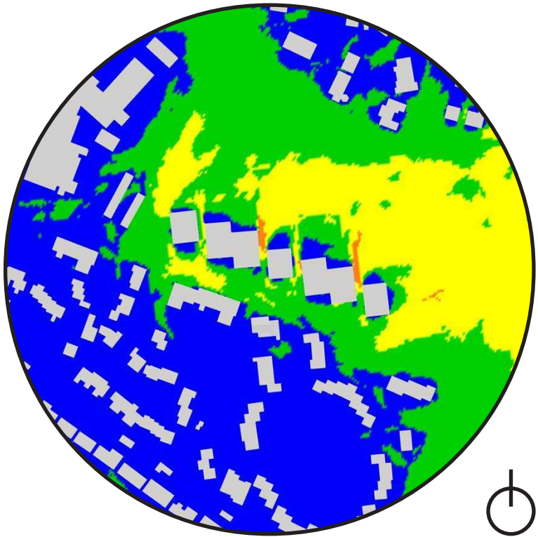
Figure 16. Lawson Comfort Contours, Existing Site with Existing Surrounds, Winter Condition
