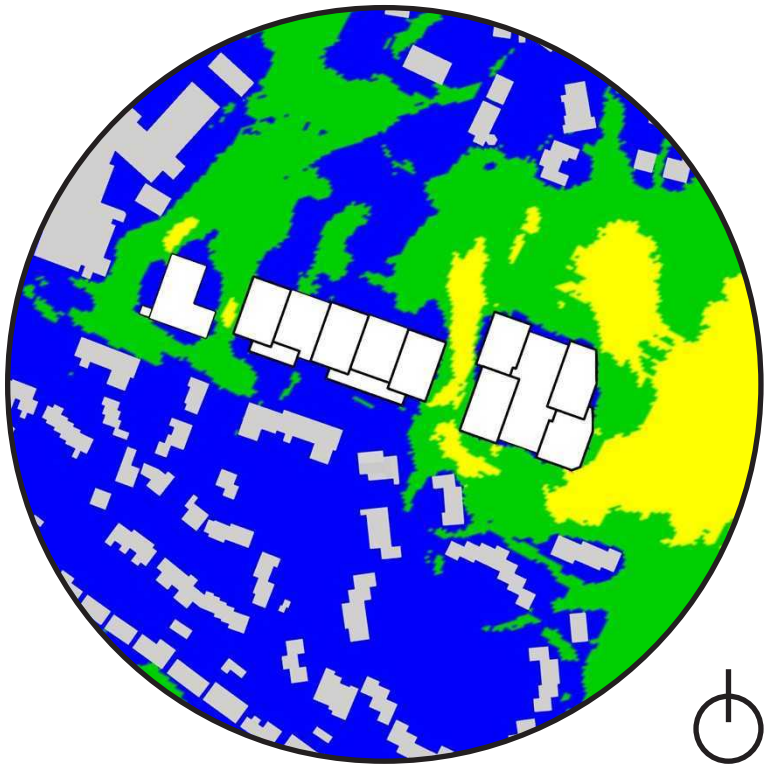
Figure 17. Lawson Comfort Contours, Proposed Site with Existing Surrounds, Winter Condition
