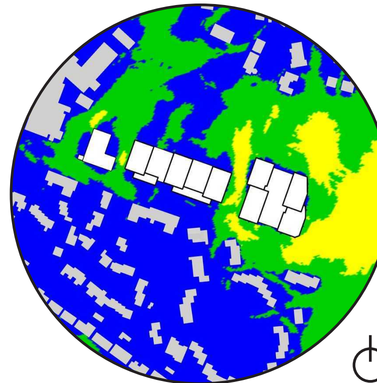
Figure 3. Lawson Comfort Contours, Proposed Site with Existing Surrounds, Winter Condition
